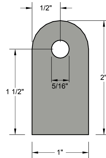
Mounting Tab Detail
